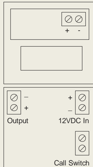
Beacon/Sounder/Reset Unit
