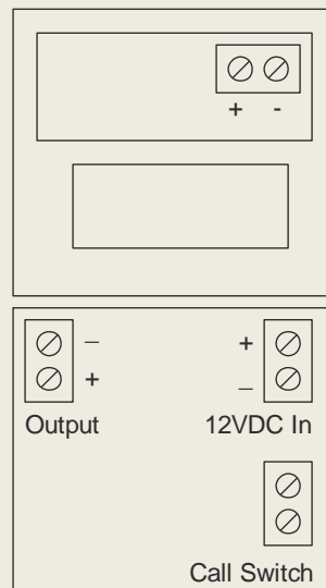
Beacon/Sounder/Reset Unit
