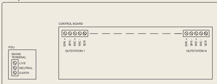
Compact Master Station
