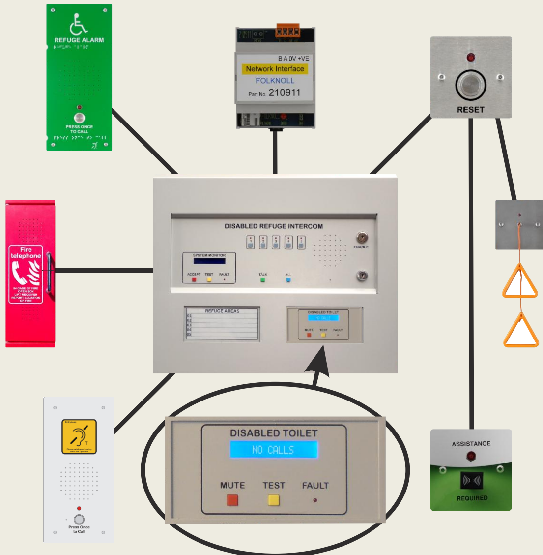
Additional displays can be mounted in the label windows.
