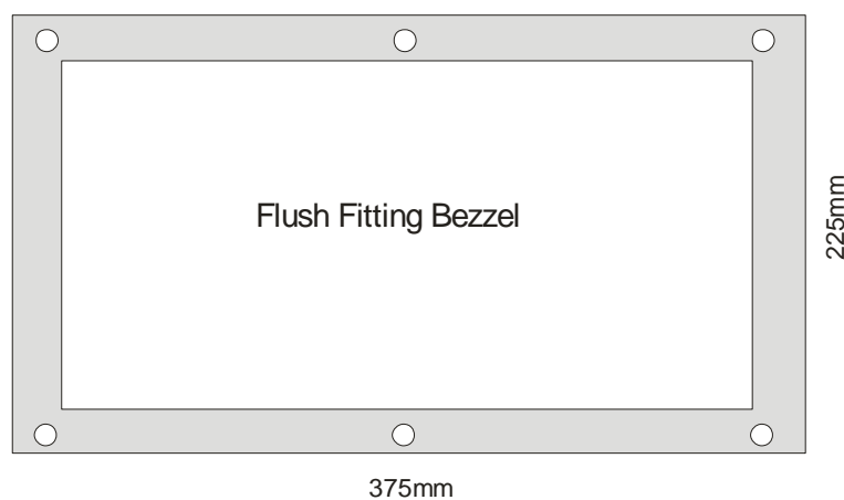
Fig 11:19 Standard System Five Way Master Station Dimensions
