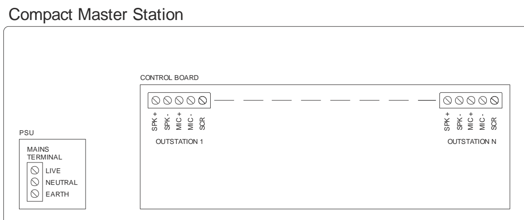
Fig 11:10 Compact Master Station Connections
