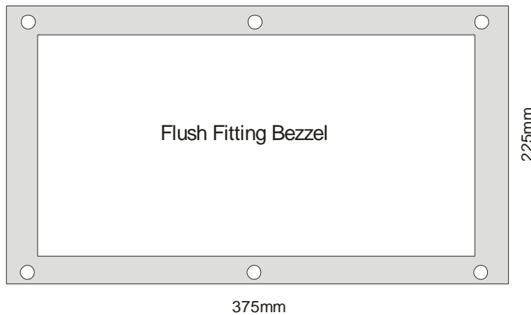
Fig 11:23 Standard System Ten Way Master Station Dimensions
