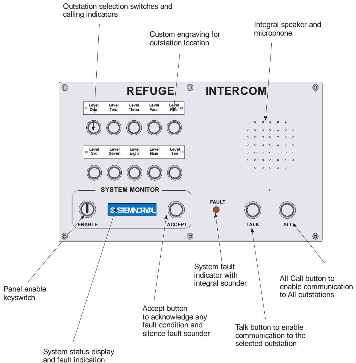
Fig 11:22 Standard System Ten Way Master Station Features
