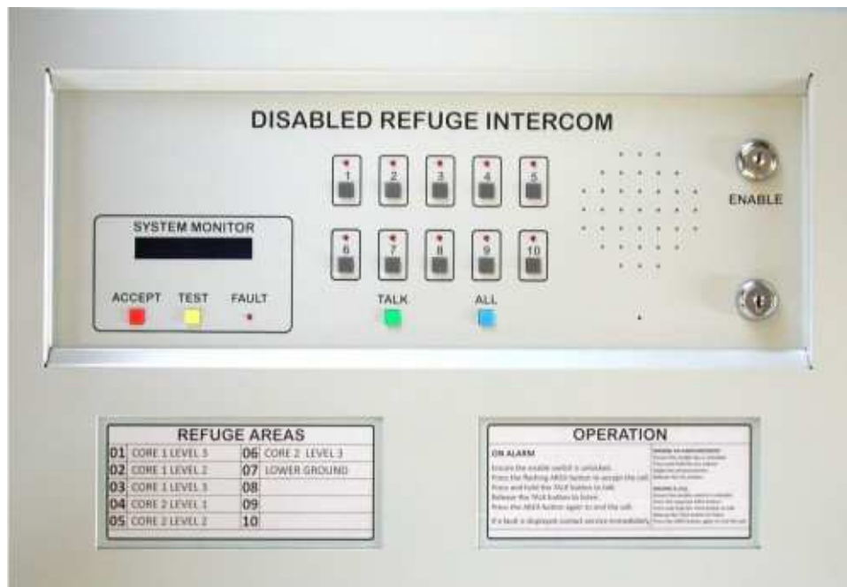
Fig 11:13 Compact System Ten Way Master Station
