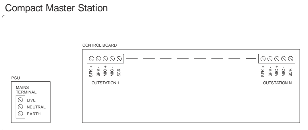
Fig 11:14 Compact Master Station Connections
