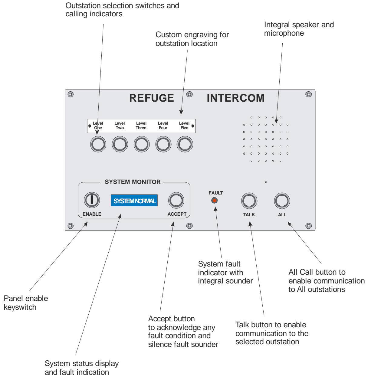
Fig 11:18 Standard System Five Way Master Station Features
