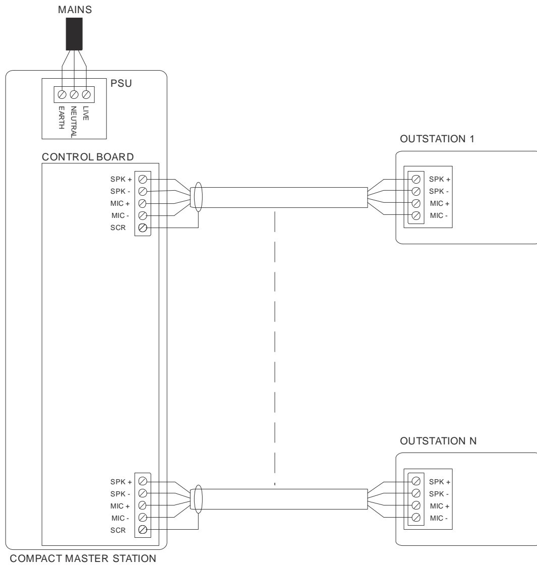
Fig 2:4 Typical Compact System Connections
