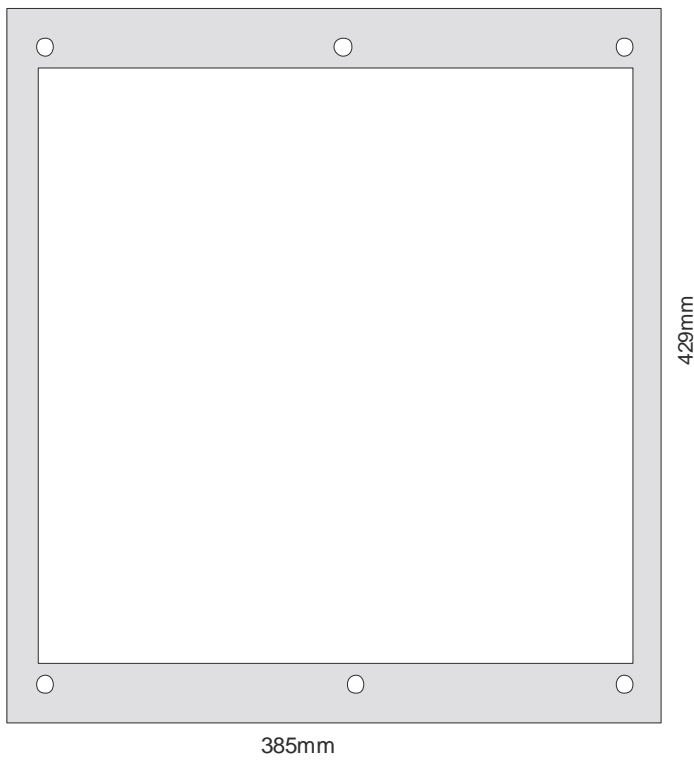
Fig 11:31 Standard System Twenty Way Master Station Dimensions
