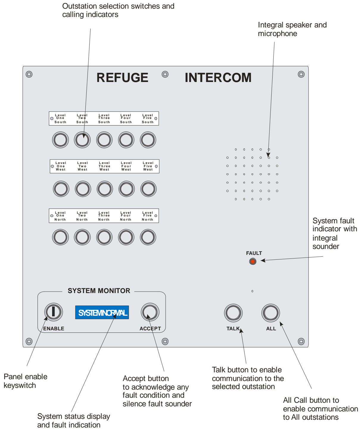
Fig 11:26 Standard System Fifteen Way Master Station Features
