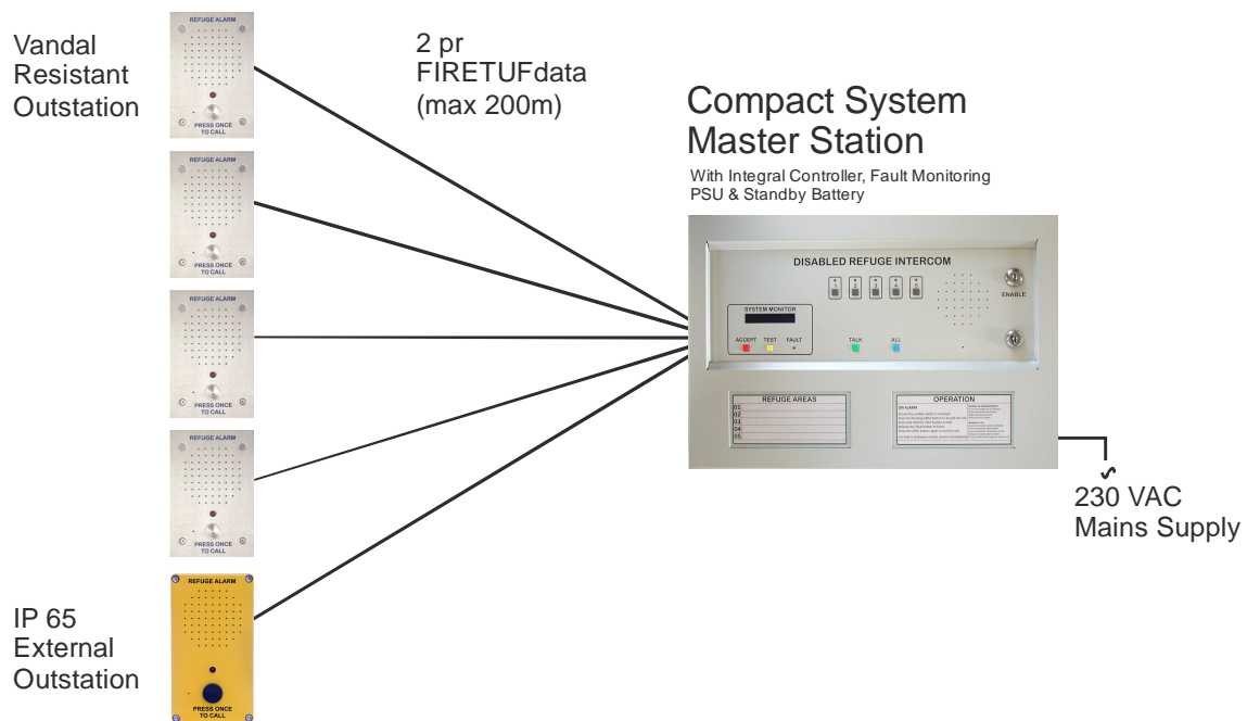
Fig 2:1 Typical Compact Disabled Refuge EVC System
