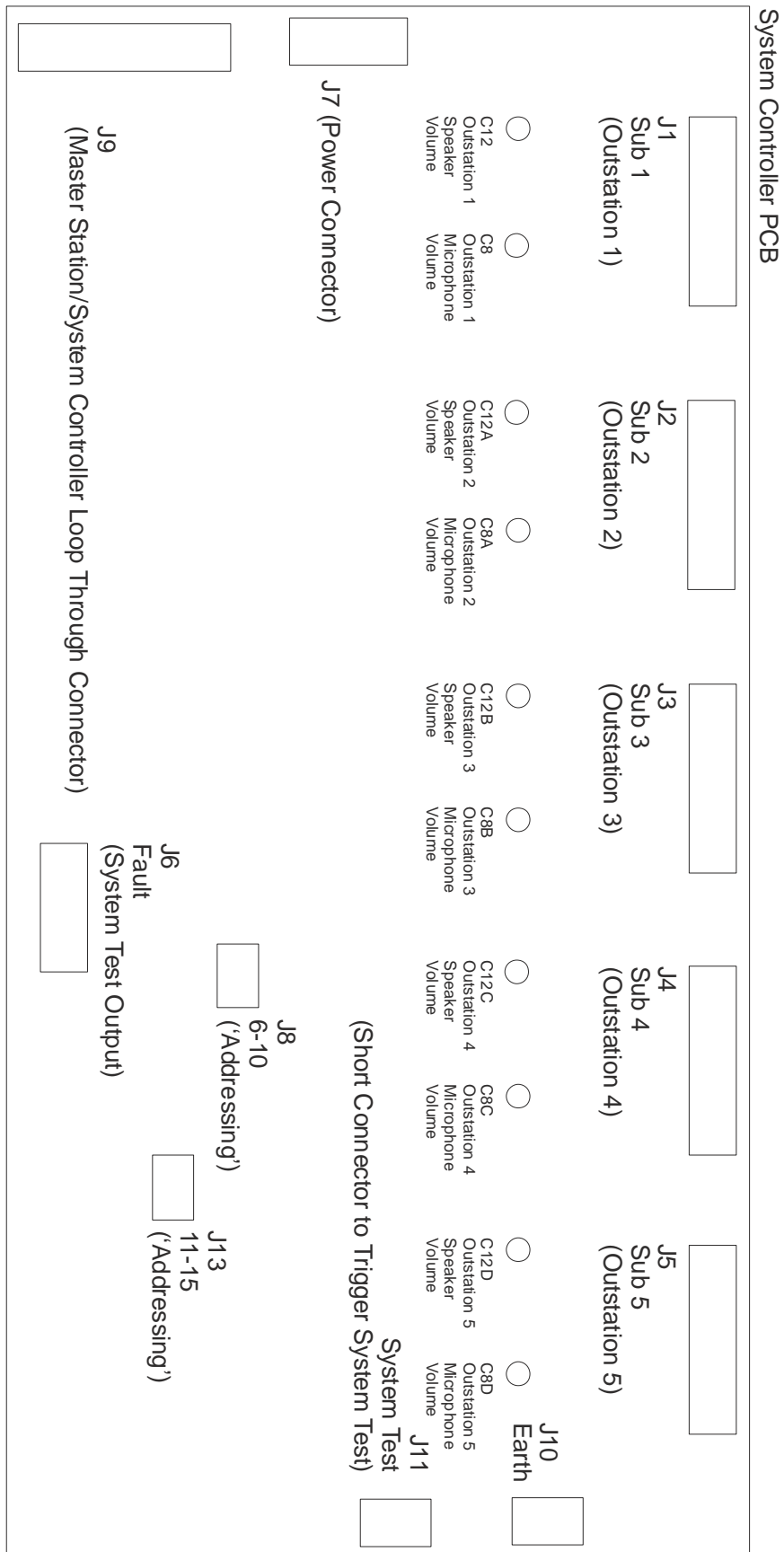
Fig 11:35 Standard System Controller PCB Layout
