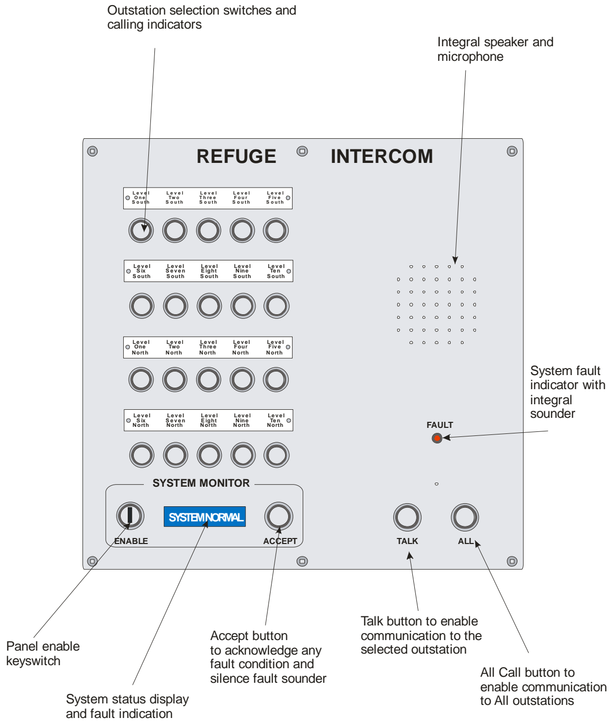
Fig 11:30 Standard System Twenty Way Master Station Features
