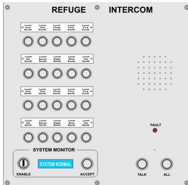
Fig 11:29 Standard System Twenty Way Master Station
